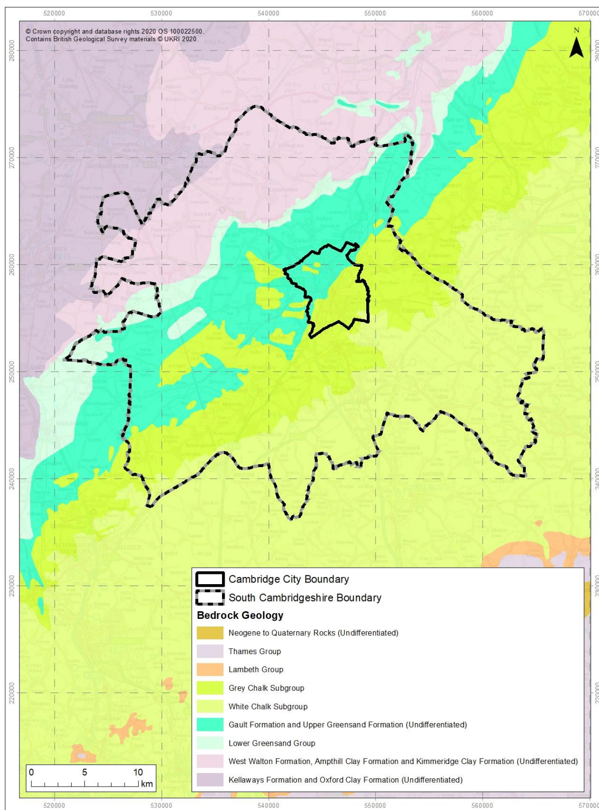
Figure 2-1: Bedrock Geology
