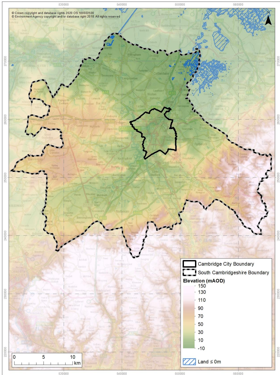
Figure 2-3: Topography
